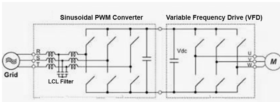
Figure 7 Diagrammatic representation of VFD with sinusoidal PWM converter (Rasin & G, 2017)
