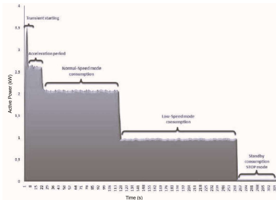
Figure 5 Several states of operating of the escalator (Uimonen, 2015)
