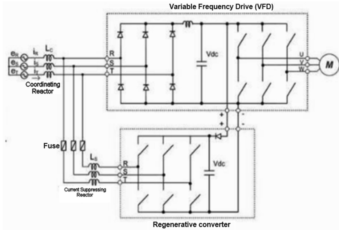
Figure 6 Diagrammatic representation of VFD with resistor brake circuit and Line Regenerative unit (Rasin & G, 2017)
