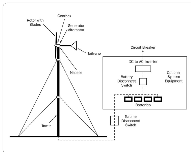
Figure 1 Components of a stand-alone wind energy system, including the electronic portion. (Clarke, 2018)
